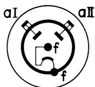
Edison-Sockel
