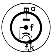
Edison-Sockel
